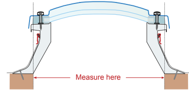
Measuring guidelines for fitting to Mardome kerb
